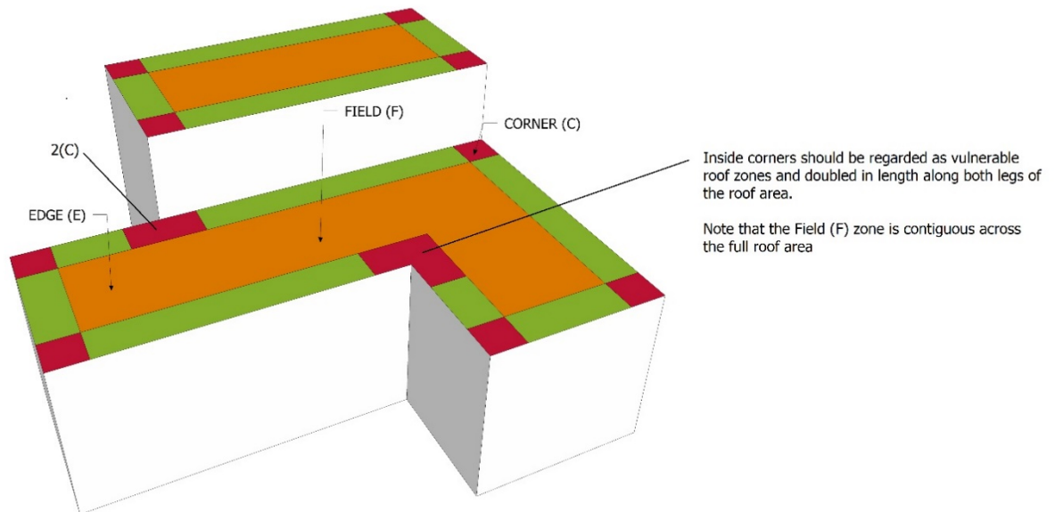
Figure 2 - NBRCA/MRGNB recommended zone layout for roof design with multiple roof heights and L-shaped building
